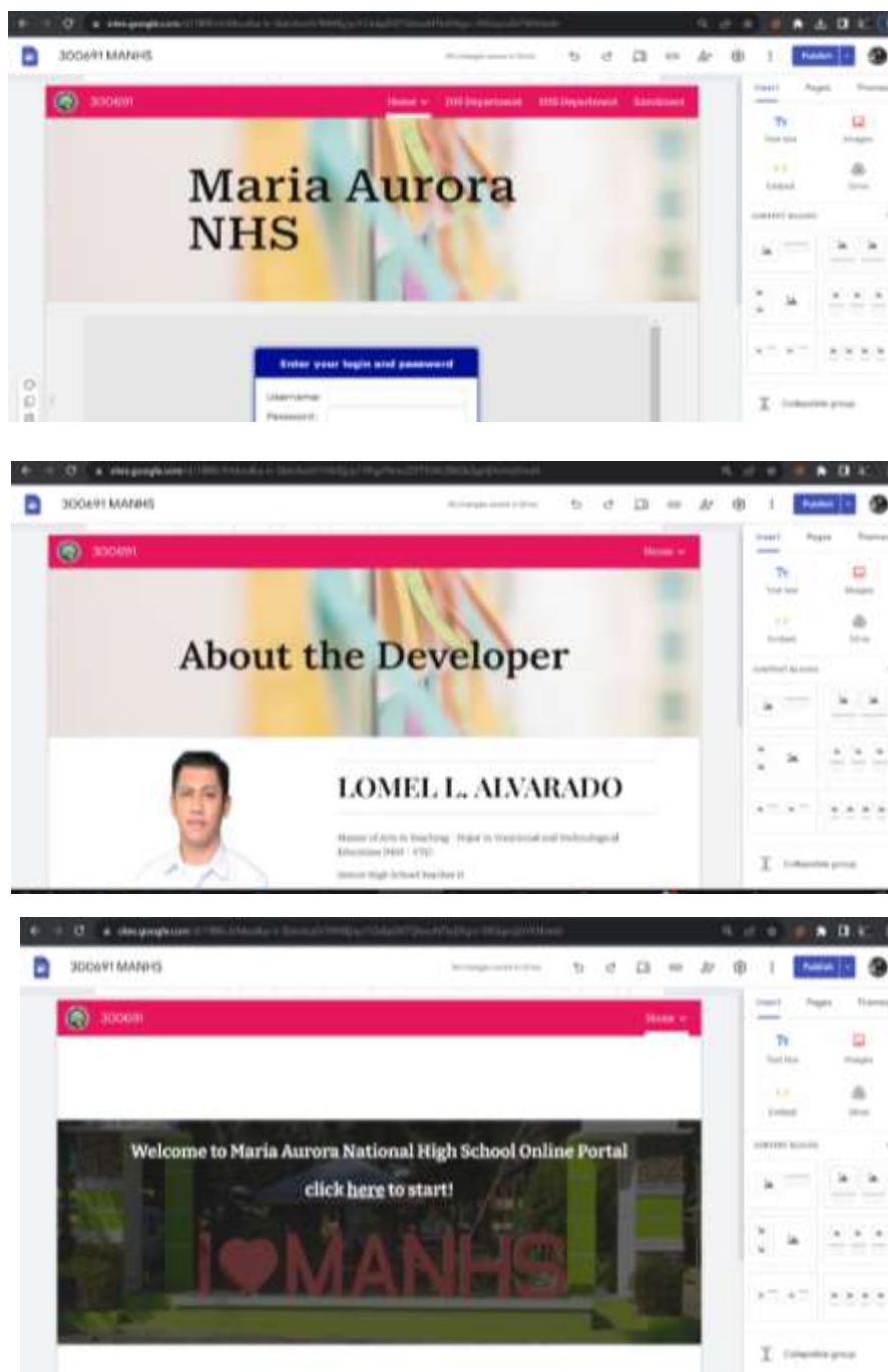
Figure 3. Developing MANHSOR
