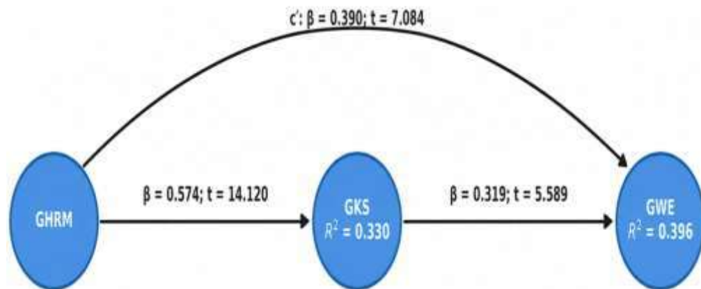
Figure 3. Bootstrap results for testing the mediating role Source: Compiled by the author
