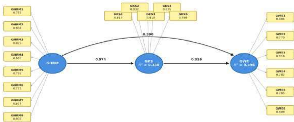
Figure 2. PLS results for the research model
